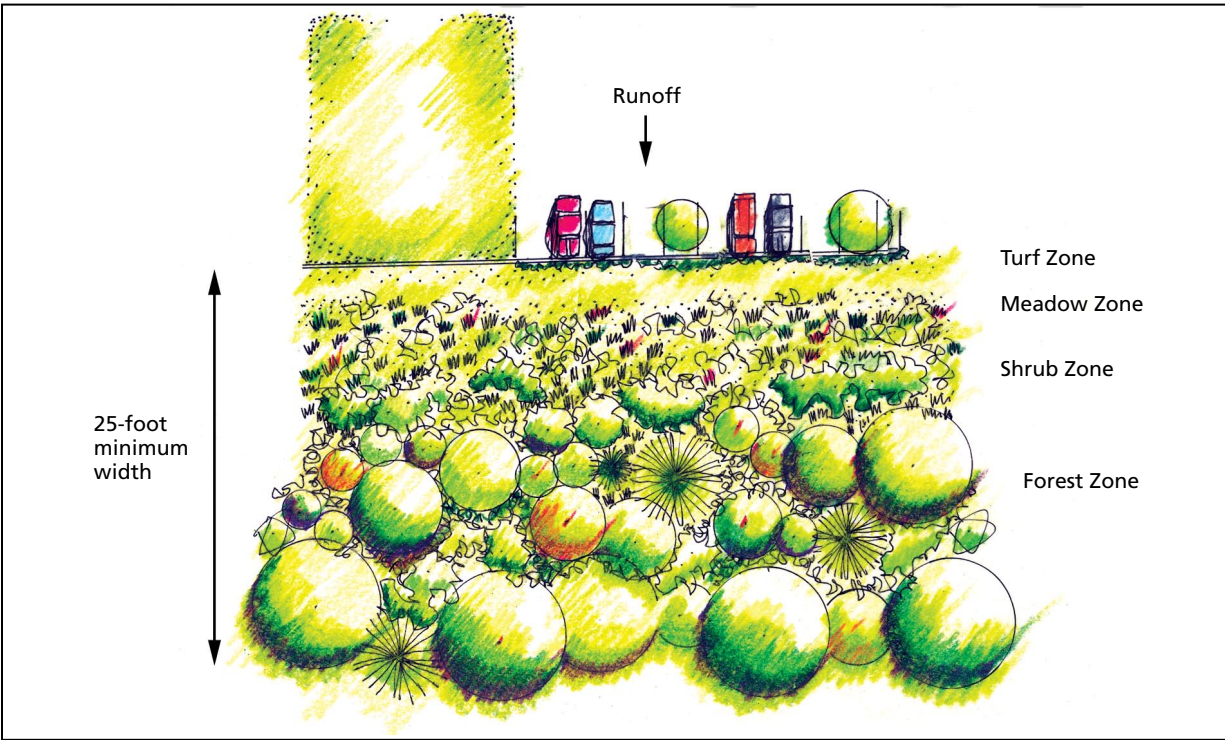
Figure 2. A multi-zone filter strip (plan) requires a minimum width of 25 feet.
