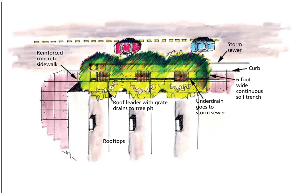
Figure 1. A linear storm water tree pit (plan view) collects and treats storm water that is directed from rooftops.
